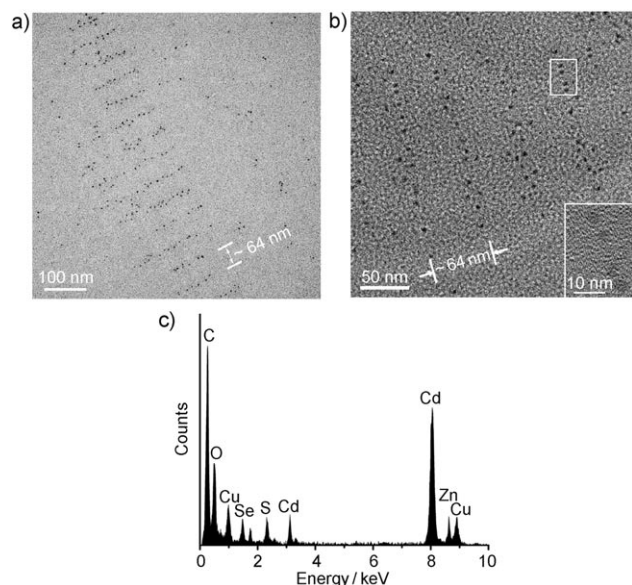
Figure 3. a) TEM image of the periodic pattern of the organized QD arrays. b) High-resolution TEM image (with a close-up inset) that reveals the crystalline structure of the QDs. c) EDX spectrum that verifies the composition of the CdSe/ZnS QDs.
